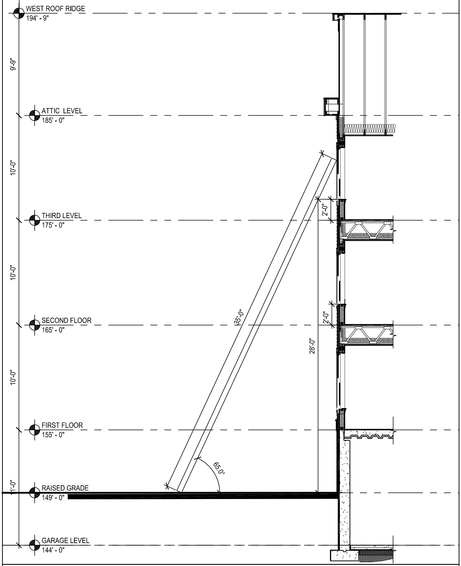
COOLIDGE AT SUDBURY - PHASE 2 Raised Grade / Fire Ladder Sketch 10.17.2016 | Scale: 3/16" = 1'-0"
